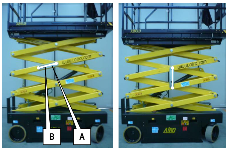
7-2: Blokkering schaarmechanisme X10 EN, X10 EW, X10 EW-WIND, XS8 E RESTYLING LIGHT, XS8 E RESTYLING
