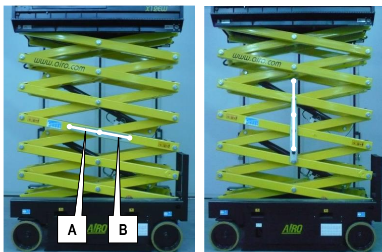
7-3: Blokkering schaarmechanisme X12 EN, X12 EW, X12 EW-WIND, X14 EW, XS9 E RESTYLING
