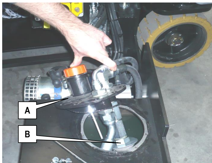
Reservoir serie XS E RESTYLING
