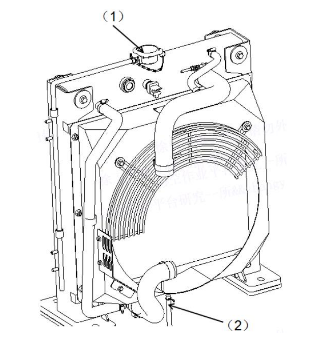
Fig.6-35 Koelvloeistof aftapopening (2).
