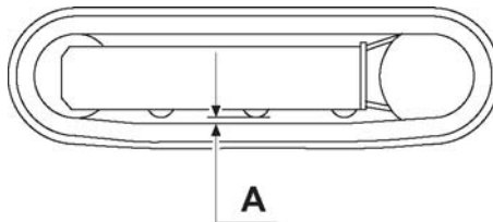
Fig. 189 Controle spanning rupsband 1
