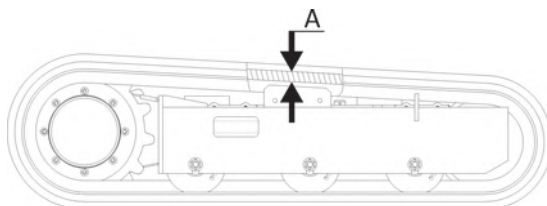
Fig. 162 Controle spanning rupsband 2
